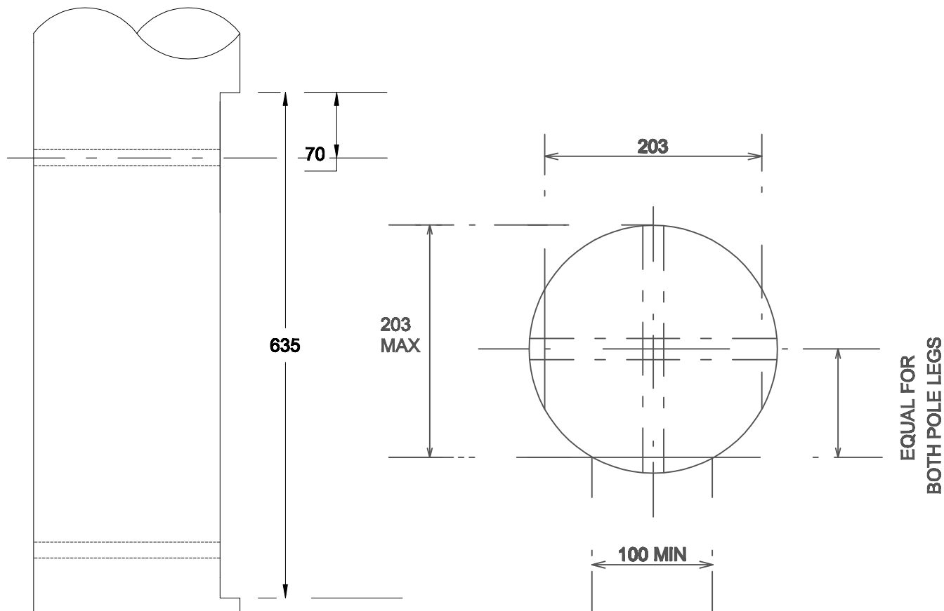
PLAN DETAIL 'A' SCALE 1:5
